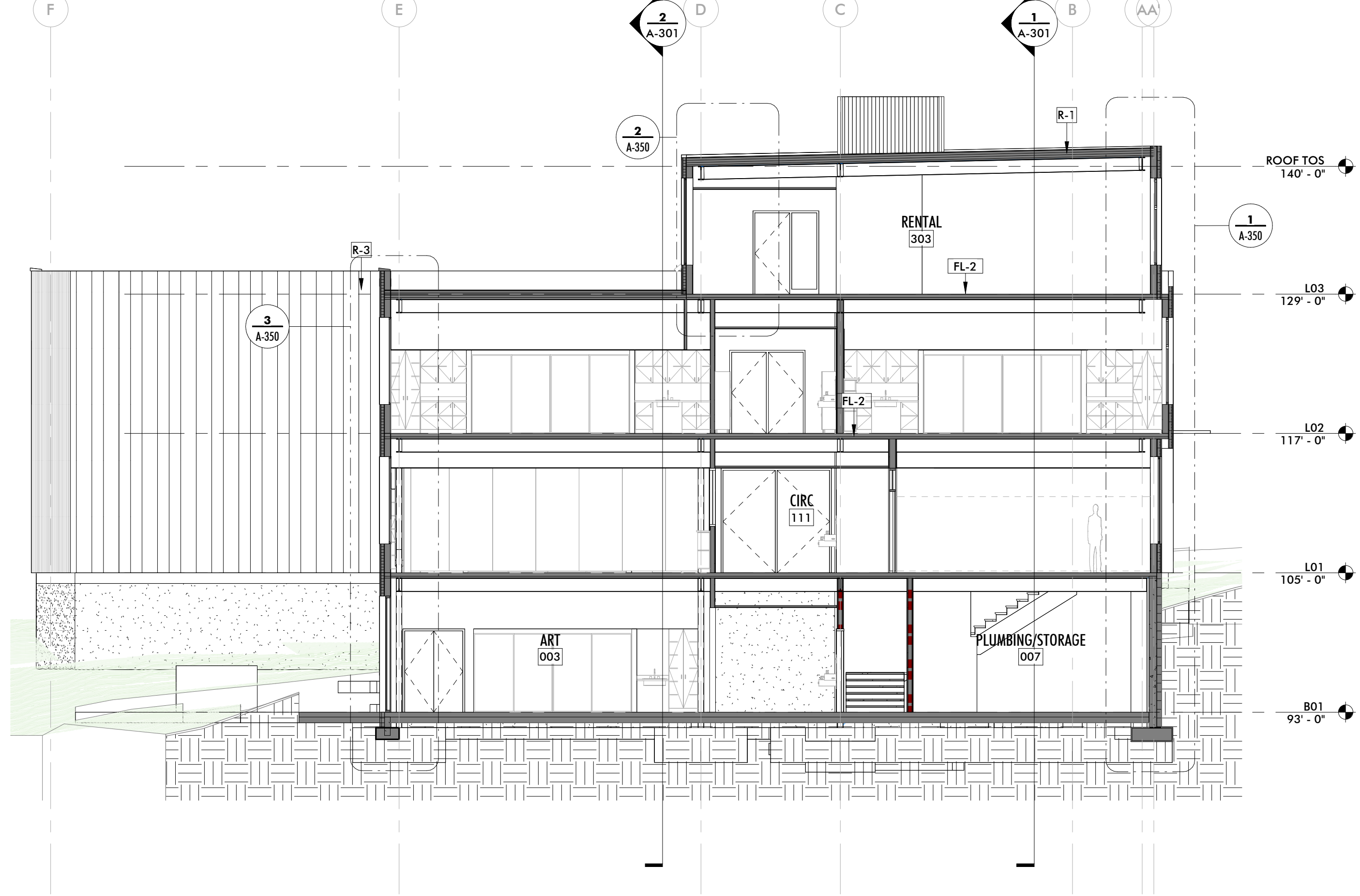
4 NORTH-SOUTH SECTION AT GRID 13 1/8" = 1'-0"
