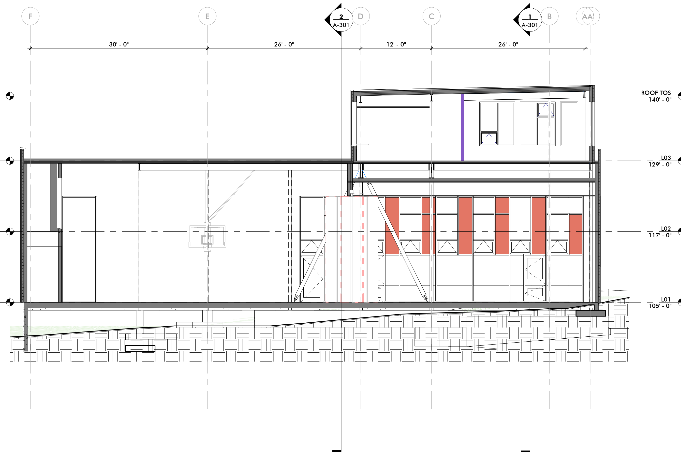
1 NORTH-SOUTH SECTION THROUGH MULTIPURPOSE & MUSIC 1/8" = 1'-0"
