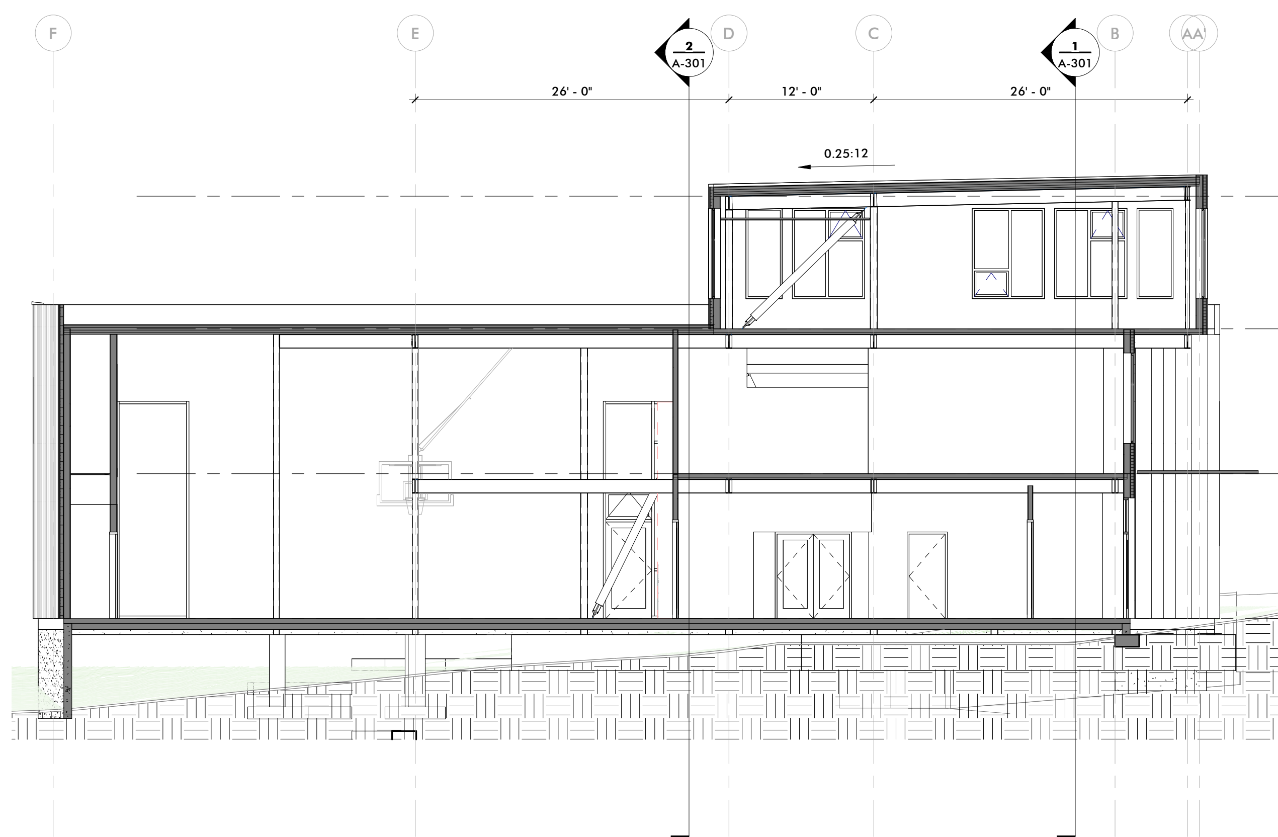
4 NORTH-SOUTH SECTION AT GRID 13 1/8" = 1'-0"
